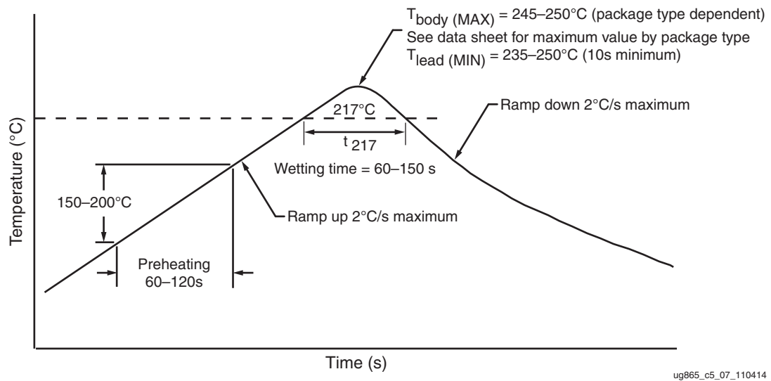
Figure 5-7: Typical Conditions for Pb-Free Reflow Soldering
