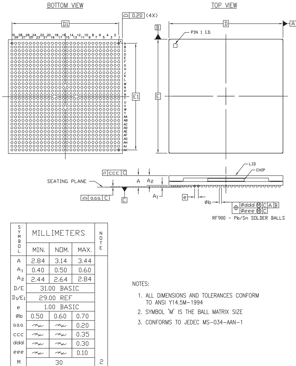
Figure 4-18: RF900 Ruggedized Flip-Chip BGA Package Specifications for the XQ7Z045 and XQ7Z100
