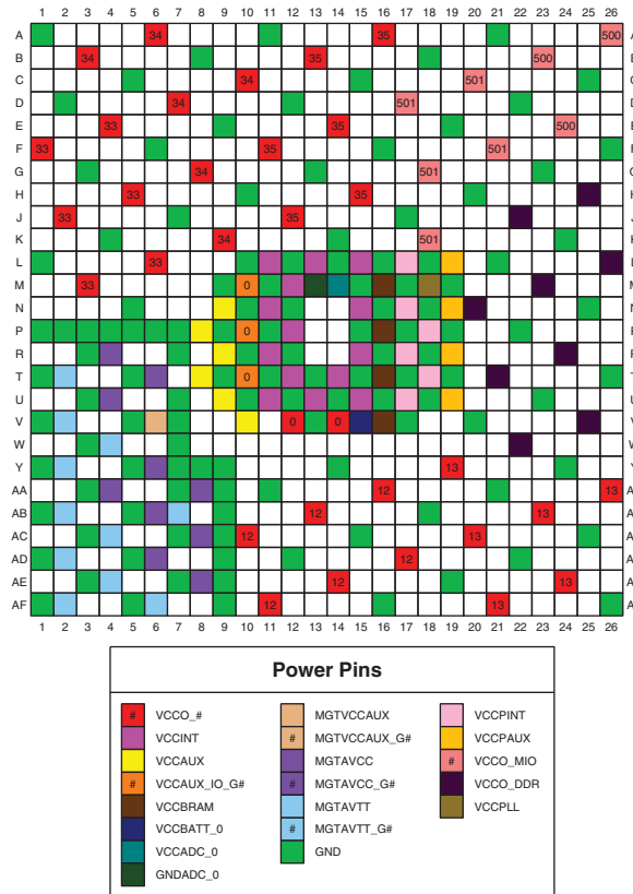
Figure 3-44: FF676/FFG676/FFV676/RF676/RFG676 Packages—XC7Z035, XC7Z045, and XQ7Z045 Power and GND Placement
