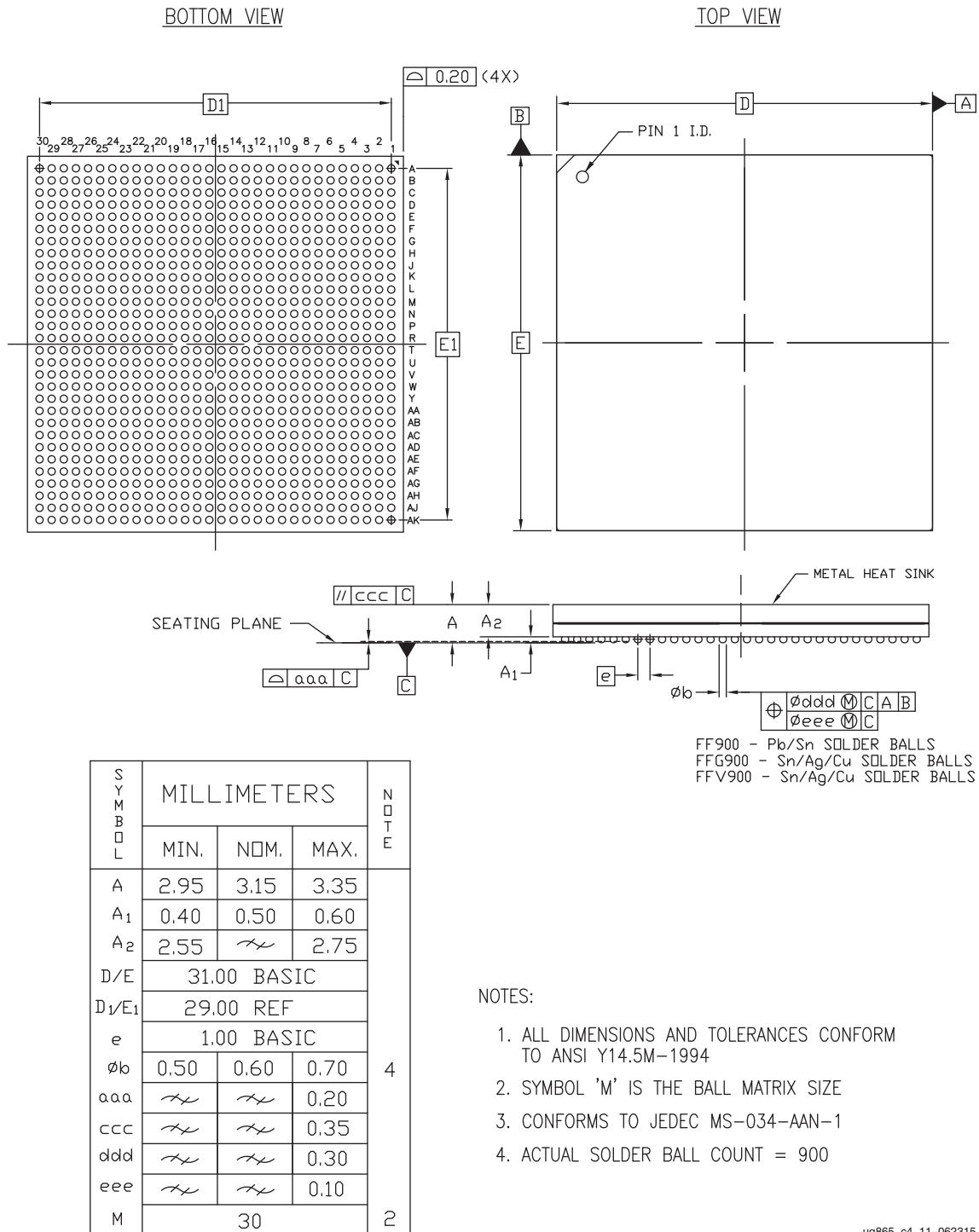
Figure 4-14: FFG900/FFV900 (XC7Z035, XC7Z045, and XC7Z100) Flip-Chip BGA Package Specifications
