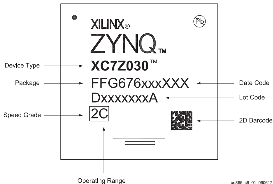
Figure 6-1: Zynq-7000 SoC Device Package Marking
