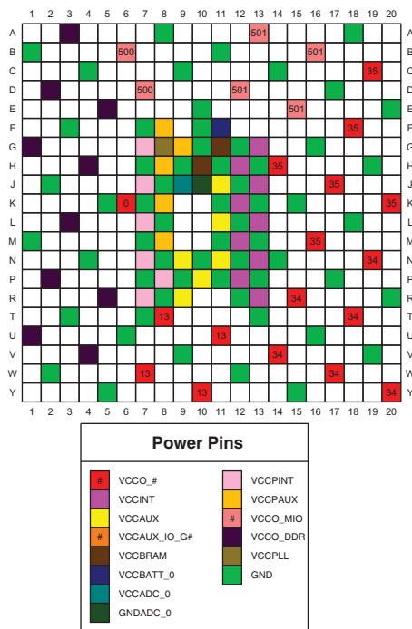
Figure 3-8: CL400/CLG400 Packages—XC7Z007S, XC7Z010, and XA7Z010 Power and GND Placement
