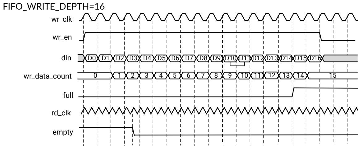
Figure 7: Standard Write Operation with Empty De-Assertion
