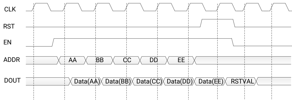
DPROM with Read Latency of 1
