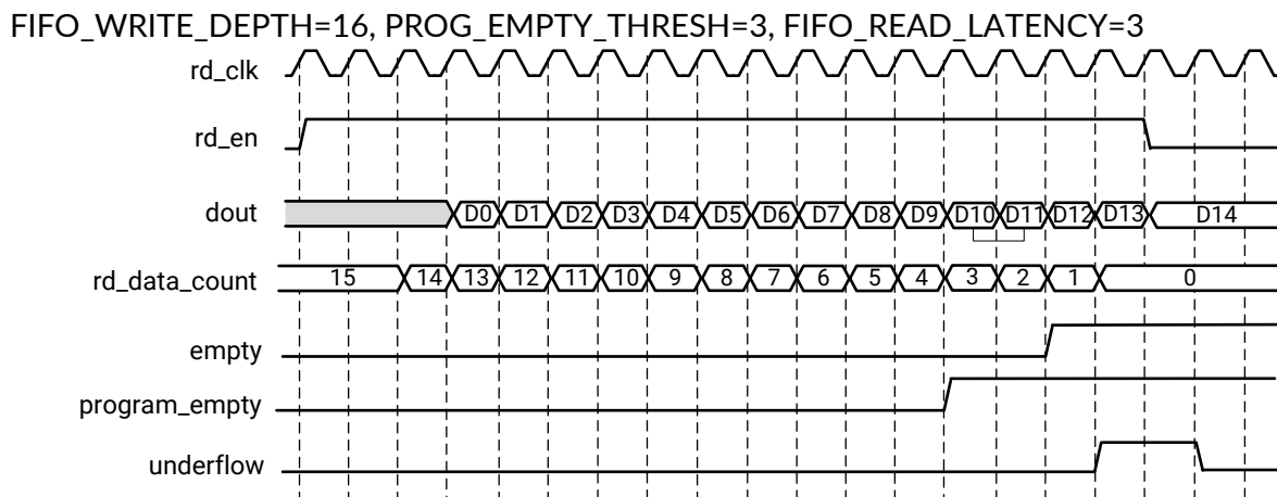
Figure 4: Standard Read Operation
