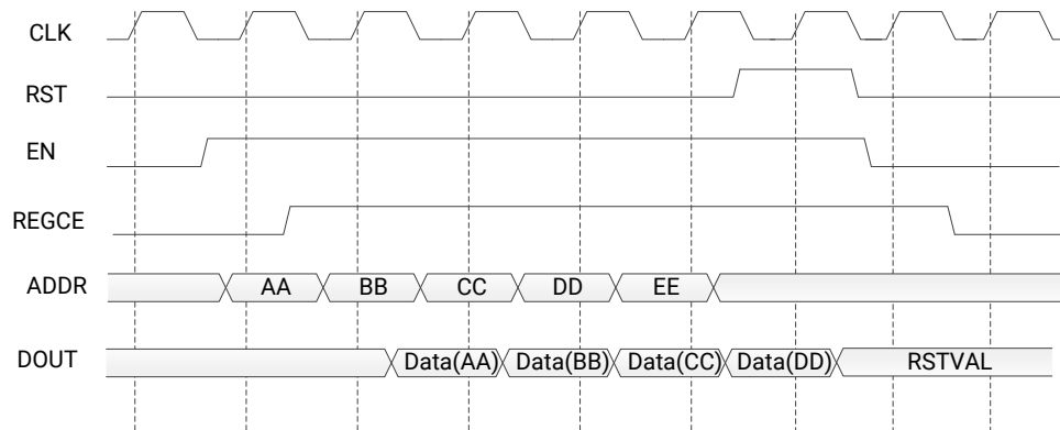
DPROM with Read Latency of 2
