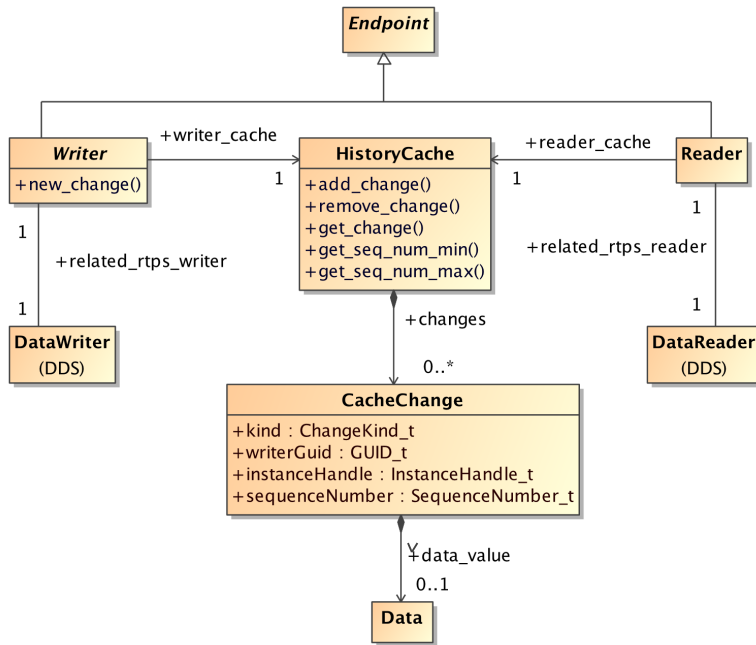
Figure 8.3 - RTPS HistoryCache
