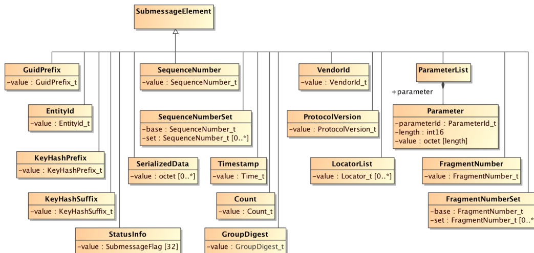
Figure 8.12 - RTPS SubmessageElements
