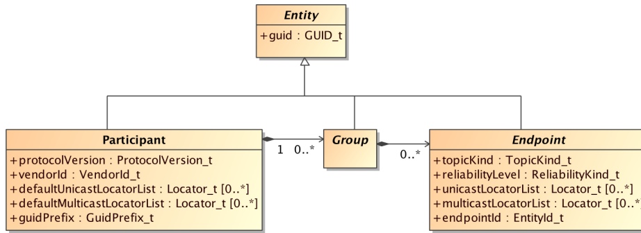
Figure 8.5 - RTPS Participant
