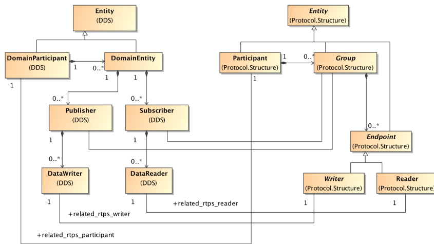
Figure 7.3 - Correspondence between RTPS and DDS Entries
