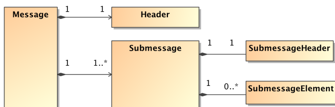
Figure 7.4 - RTPS Messages Module
