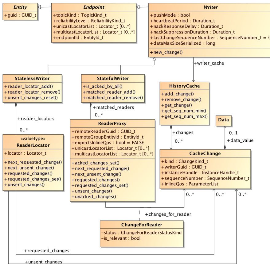
Figure 8.15 - RTPS Writer Endpoints
