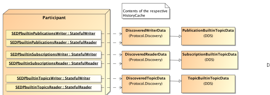
Figure 8.31 - Built-in Endpoints and the DataType associated with their respective HistoryCache
