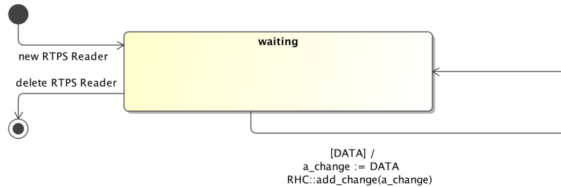
Figure 8.22 - Behavior of the Best-Effort StatelessReader
