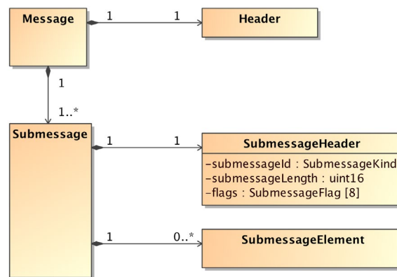
Figure 8.10 - Structure of the RTPS Submessages
