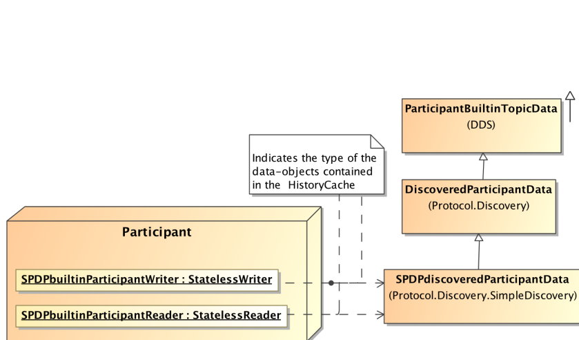
Figure 8.28 - The built-in Endpoints used by the Simple Participant Discovery Protocol
