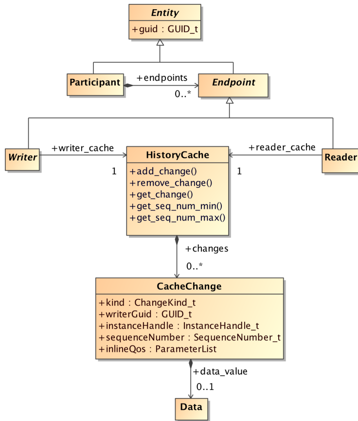
Figure 8.1 - RTPS Structure Module
