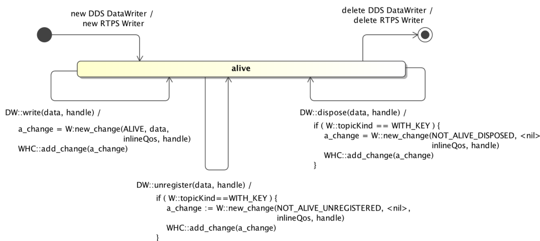
Figure 8.6 - DDS DataWriter additions to the HistoryCache
