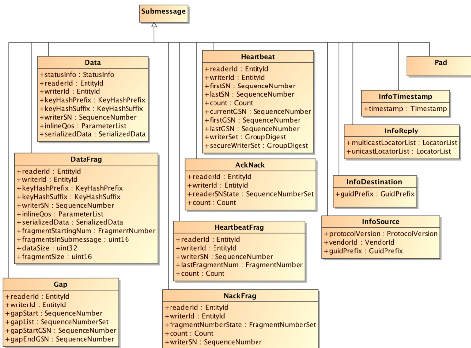
Figure 8.13 - RTPS Submessages
