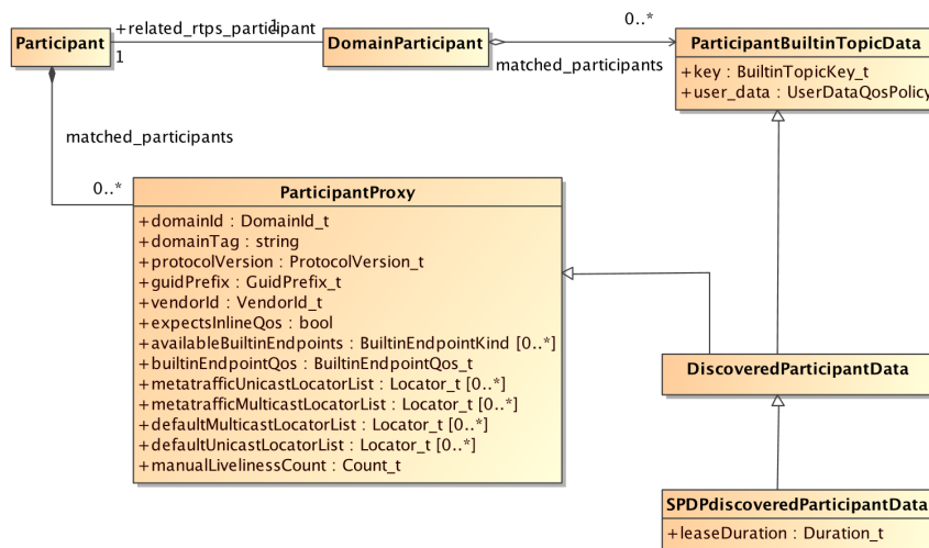
Figure 8.27 - SPDPdiscoveredParticipantData
