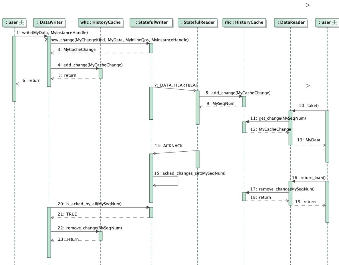
Figure 8.14 – Example Behavior
